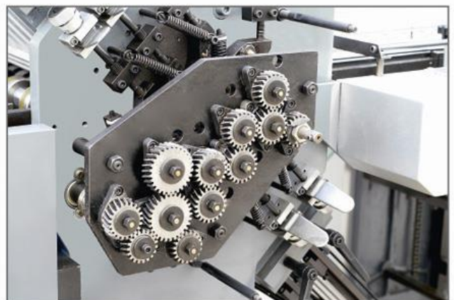
高精度的十字联轴器转动调整 High-precision Spindle Coupler Transmission
